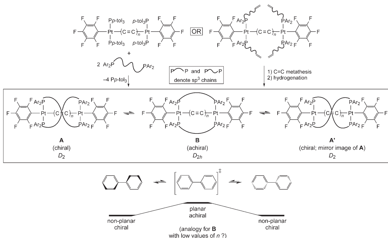
Scheme 1. Syntheses and limiting structures of complexes \text{PtC}_x\text{Pt-m/Ar} ( x=2n ) derived from \text{C}_6\text{F}_5\text{Pt}(\text{C}\equiv\text{C})_n\text{PtC}_6\text{F}_5 units and termini-spanning \alpha,\omega -diphosphines \text{Ar}_2\text{P}(\text{CH}_2)_m\text{PAr}_2 (top, middle), and approaches to destabilizing conformations with coplanar endgroups such as B (bottom).
