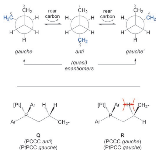
Figure 7. Some conformational issues in double-helical complexes A . An important step in enantiomer interconversion (top). Steric interactions as a function of PAR 2 CH 2 CH 2 CH 2 conformations (bottom).
