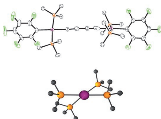
Figure 2. Partial views of the molecular structure of \text{Pt}_6\text{Pt} (ellipsoids/spheres: purple = platinum, orange = phosphorus, green = fluorine, gray = carbon).
