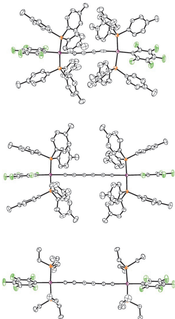
Figure 1. Thermal ellipsoid plots (50% probability level) of \text{Pt}_4\text{Pt} (top), \text{Pt}_6\text{Pt}-4\text{THF} (middle; solvate molecules omitted), and \text{Pt}_8\text{Pt} (bottom) (ellipsoids: purple = platinum, orange = phosphorus, green = fluorine, gray = carbon).
