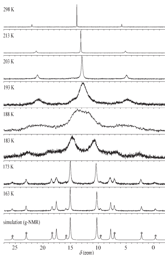
Figure 6. Variable-temperature ^{31}\text{P}\{^1\text{H}\} NMR spectra of \text{PtC}_4\text{Pt-8/Ph} (162 MHz, [\text{D}_8]\text{THF} ; * denotes a platinum satellite).
